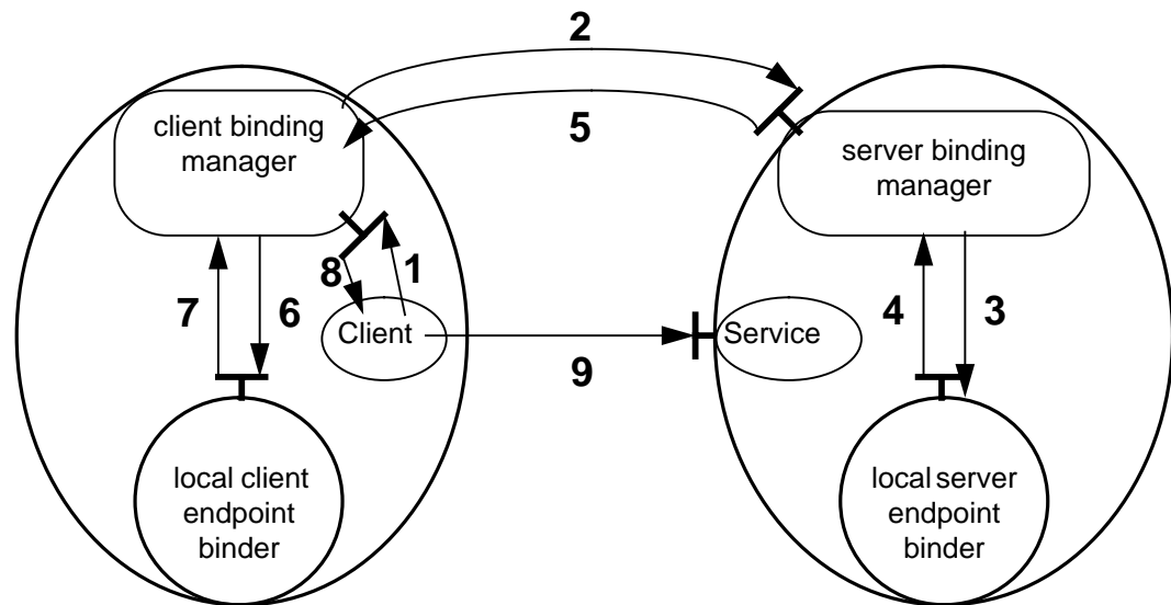
Figure 7.2: Using both client and server binding managers
