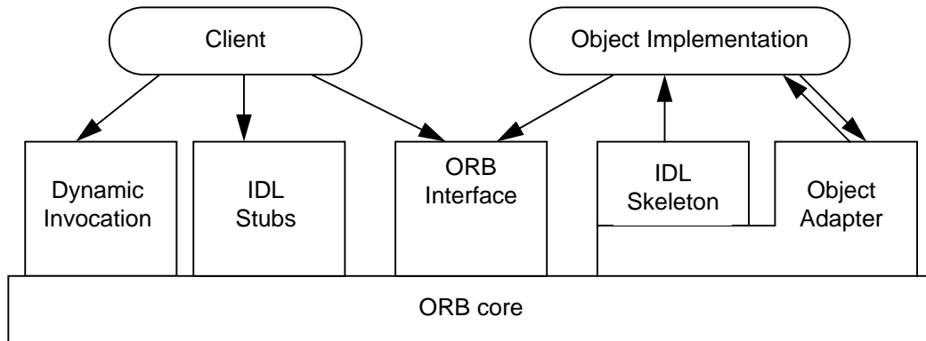
Figure 3.1: CORBA Components
