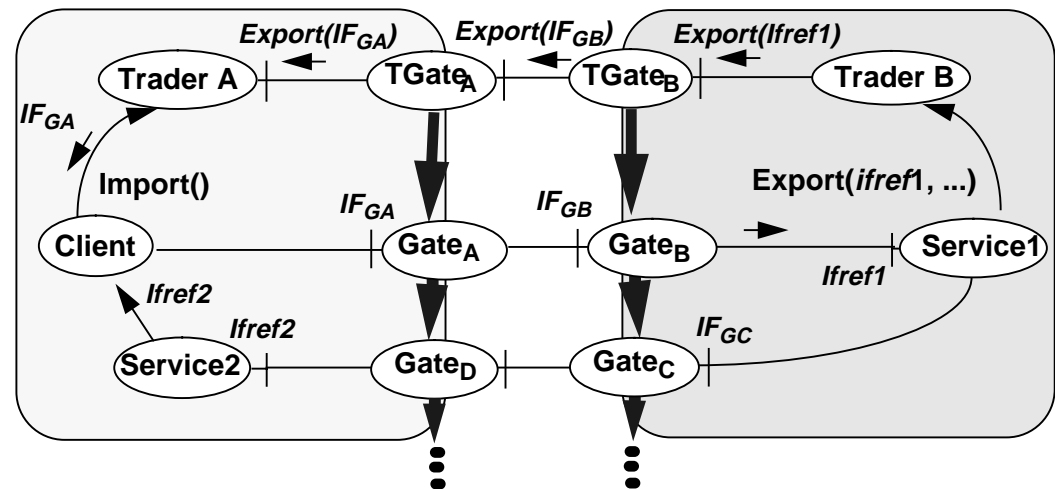
Figure 8.5: Computational model of interception: the cloning nature of setting up the gateways
