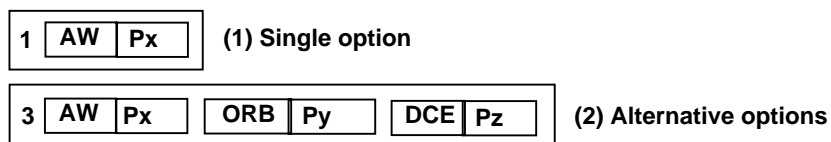
Figure 14.1: Interface Reference structure - one or more alternative paths
